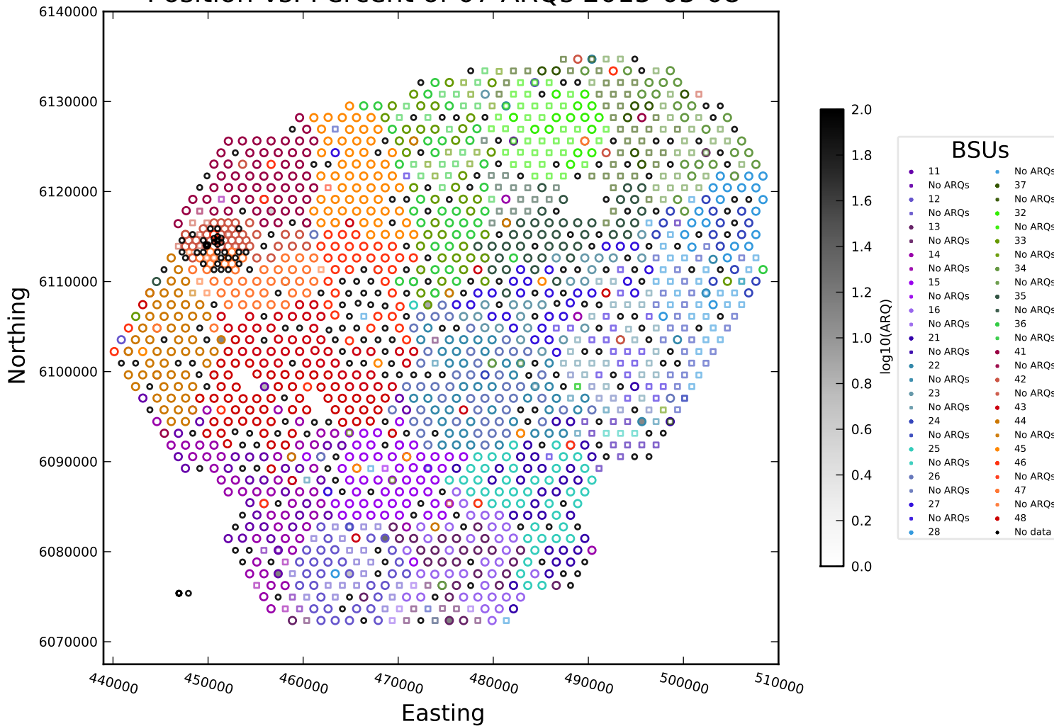
Position vs. Percent of 07 ARQs 2015-05-08
