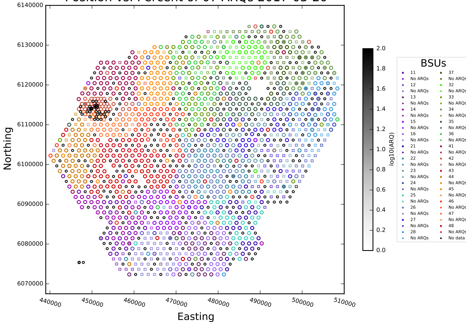
Position vs. Percent of 07 ARQs 2017-03-20
