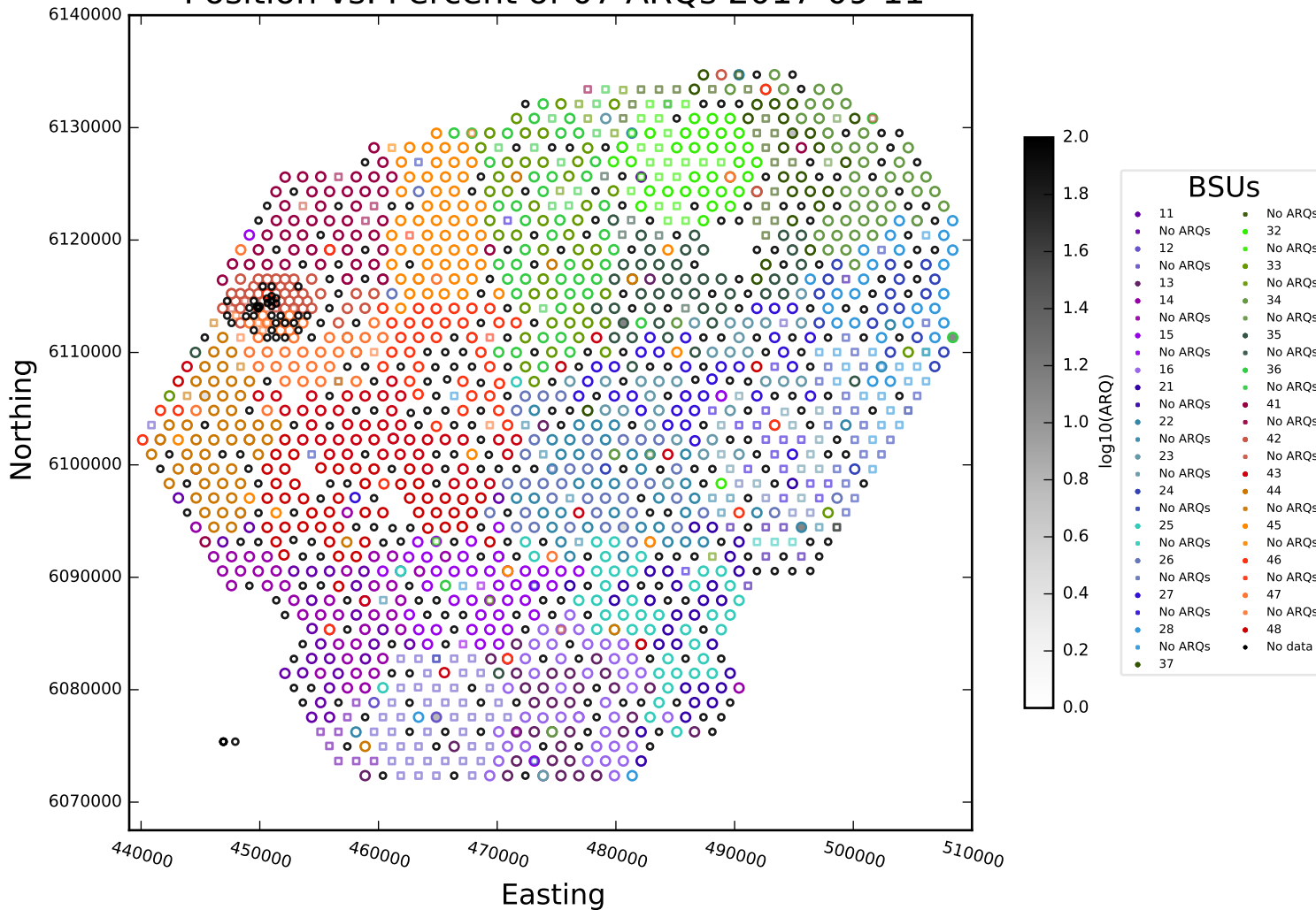
Position vs. Percent of 07 ARQs 2017-09-11
