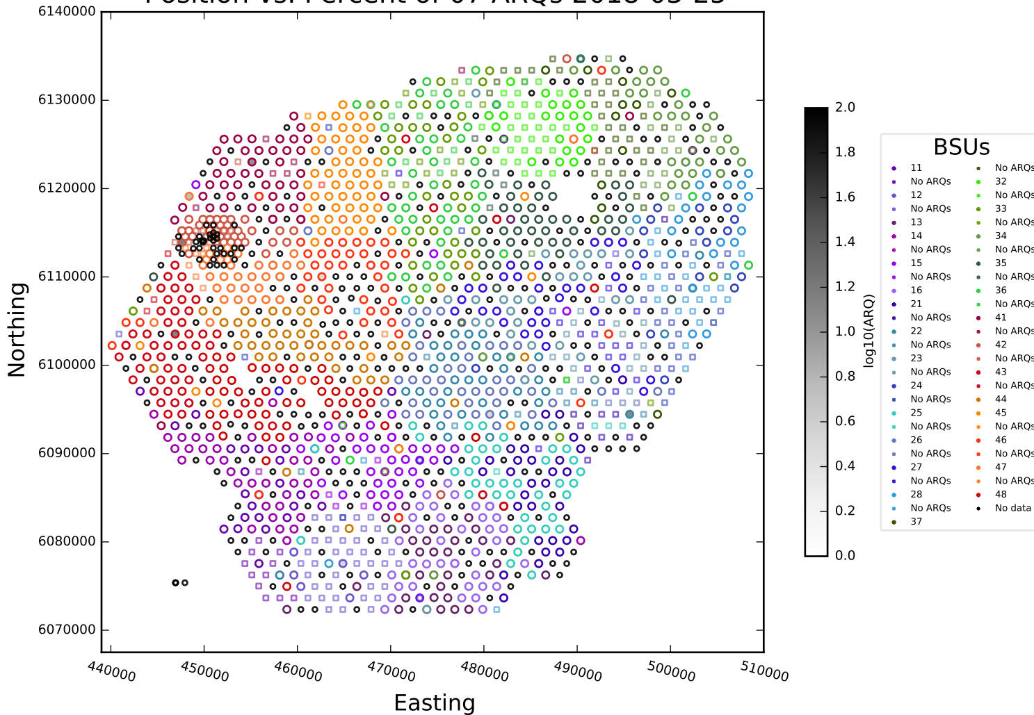
Position vs. Percent of 07 ARQs 2018-03-25
