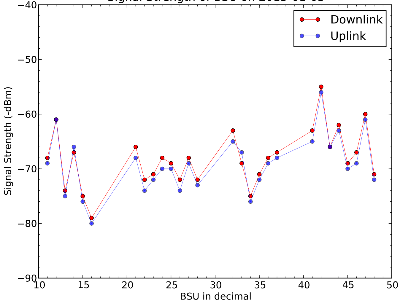
Signal Strength of BSU on 2015-01-03
