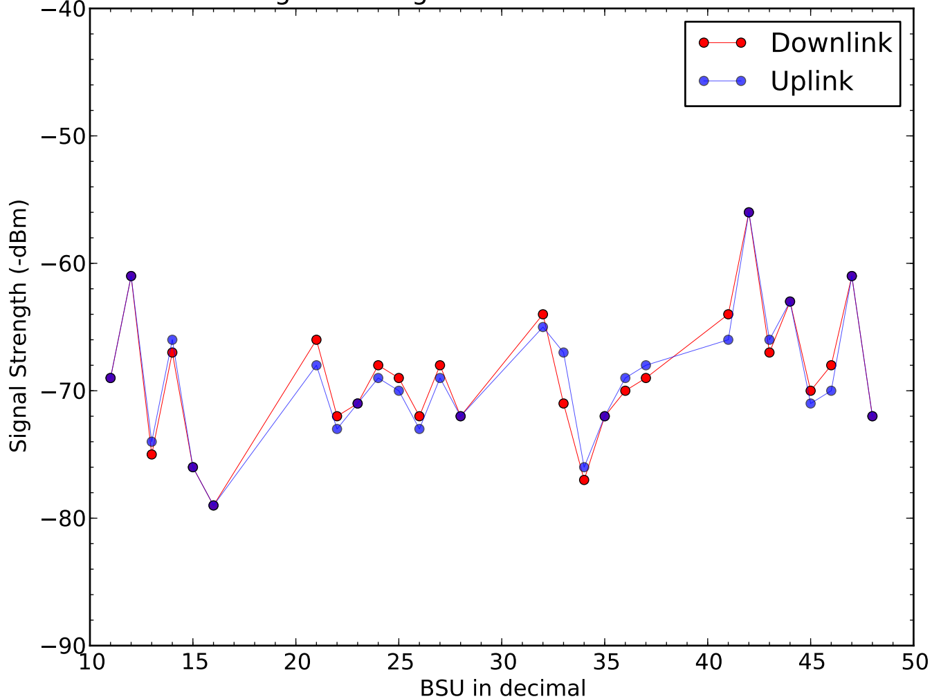
Signal Strength of BSU on 2015-01-14
