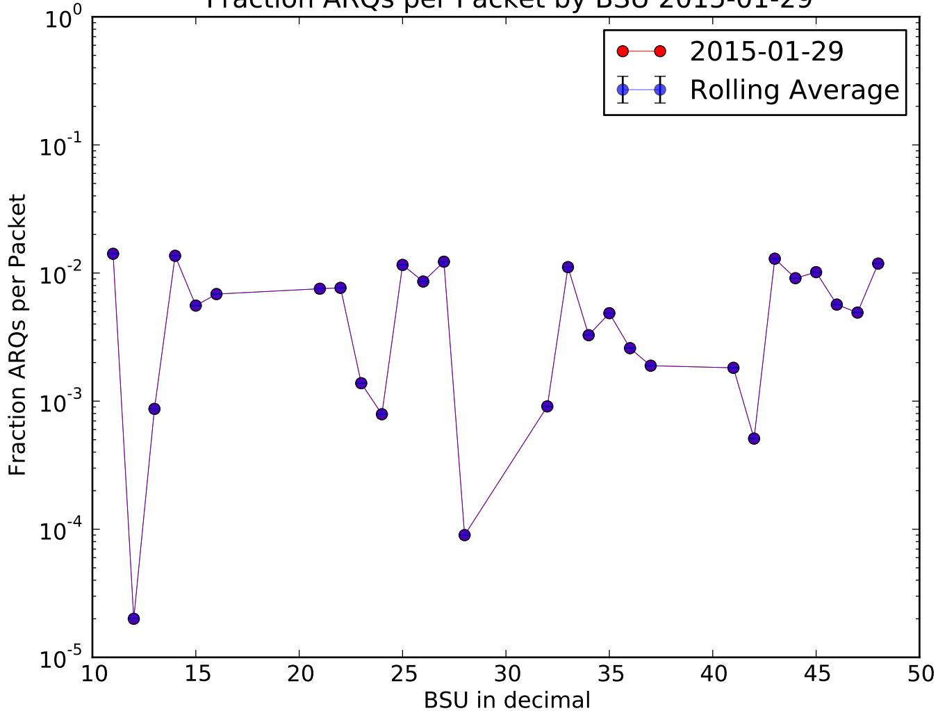
Fraction ARQs per Packet by BSU 2015-01-29
