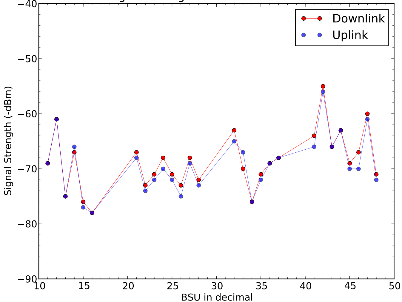
Signal Strength of BSU on 2015-01-30
