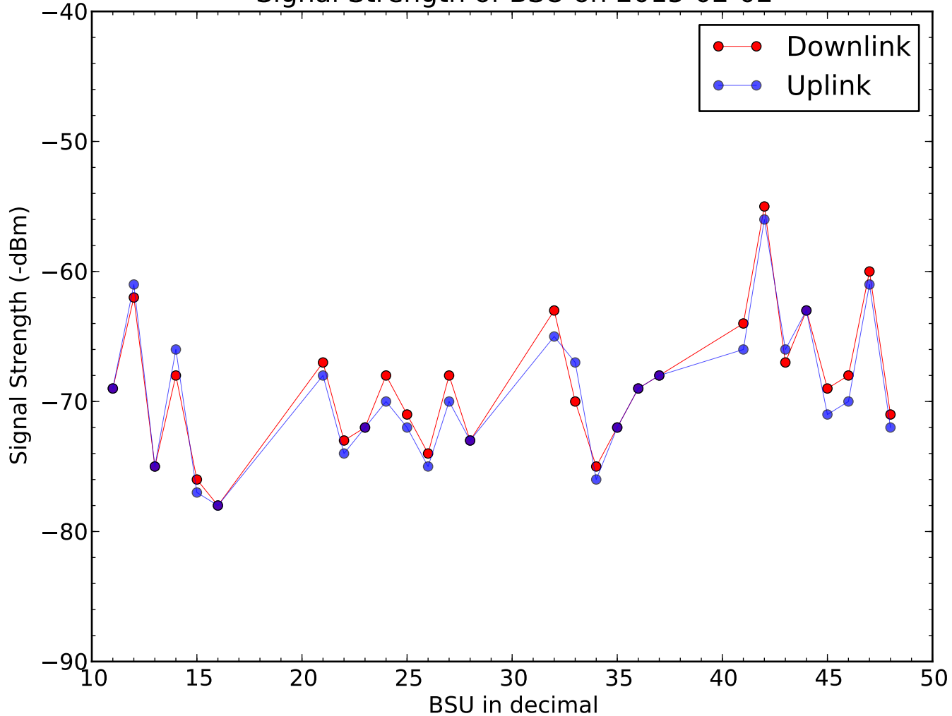
Signal Strength of BSU on 2015-02-02
