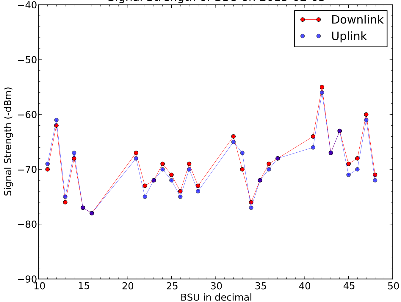
Signal Strength of BSU on 2015-02-05
