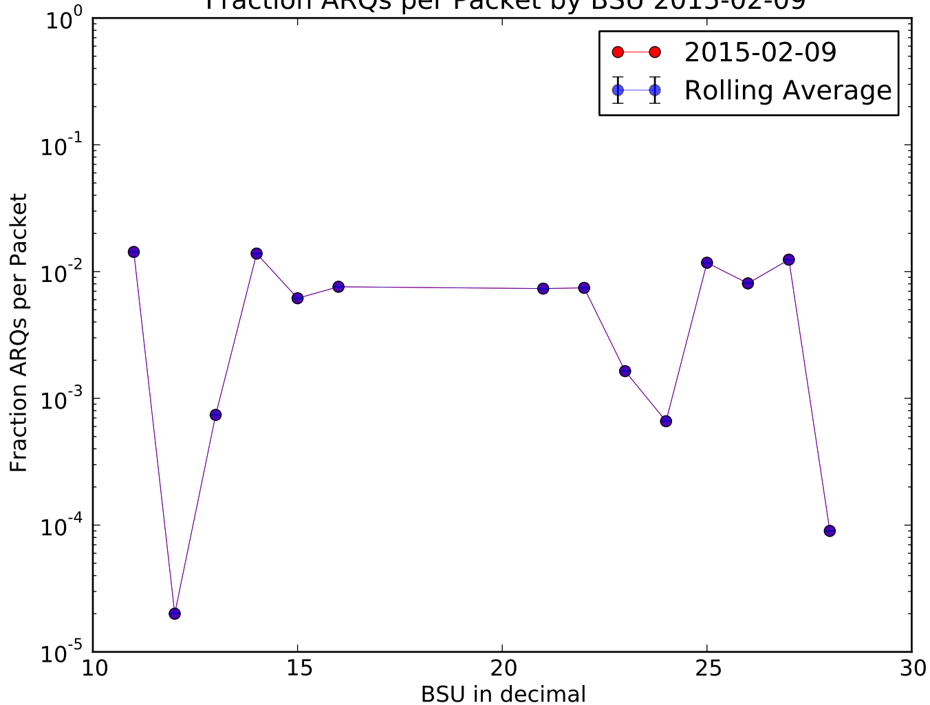
Fraction ARQs per Packet by BSU 2015-02-09
