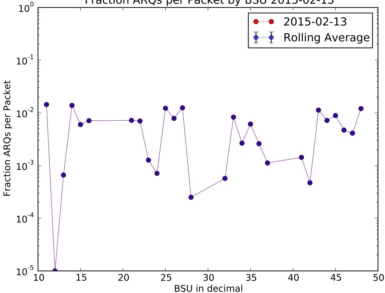
Fraction ARQs per Packet by BSU 2015-02-13
