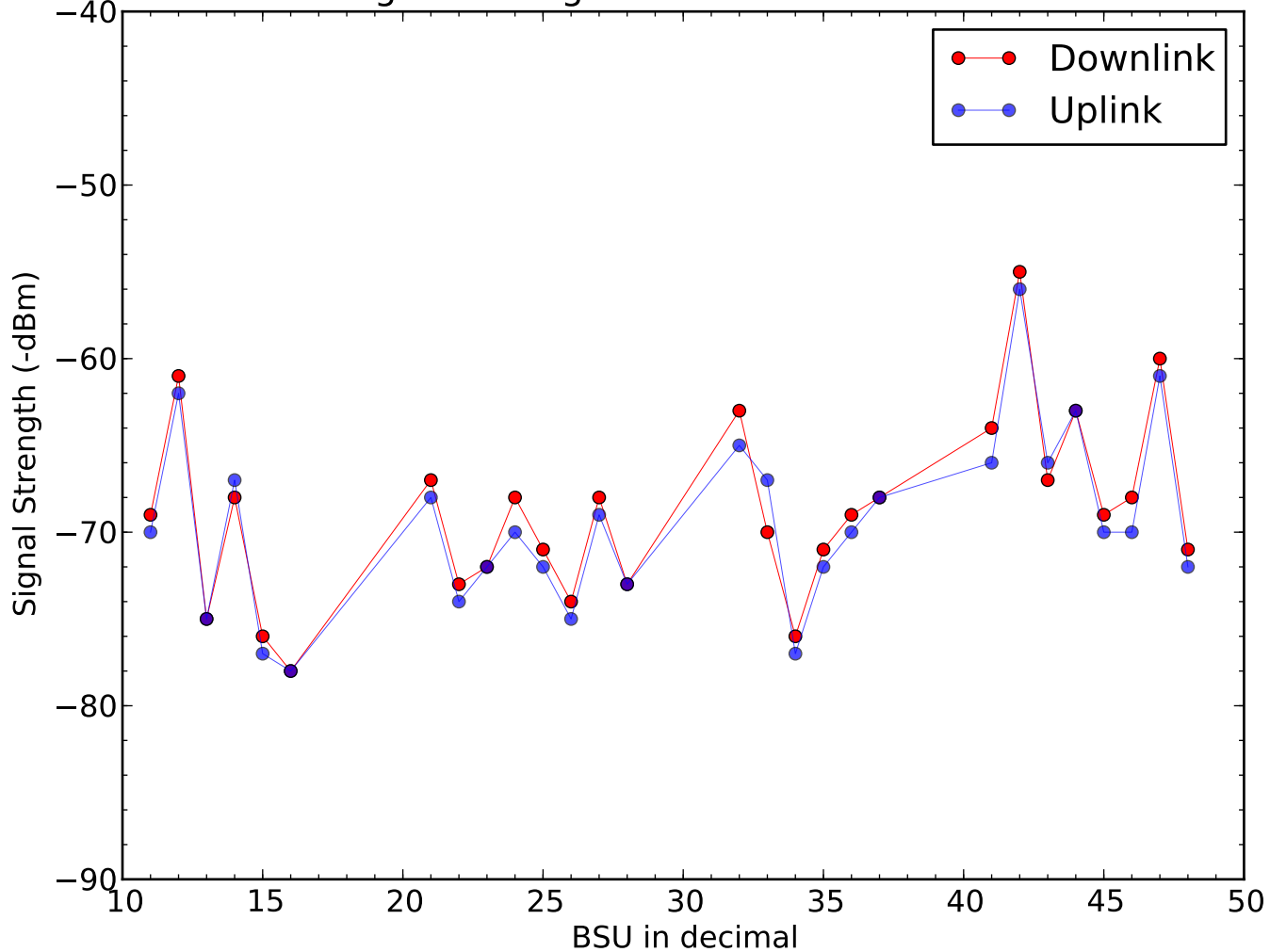
Signal Strength of BSU on 2015-02-15
