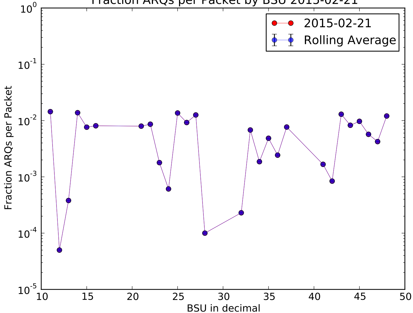
Fraction ARQs per Packet by BSU 2015-02-21
