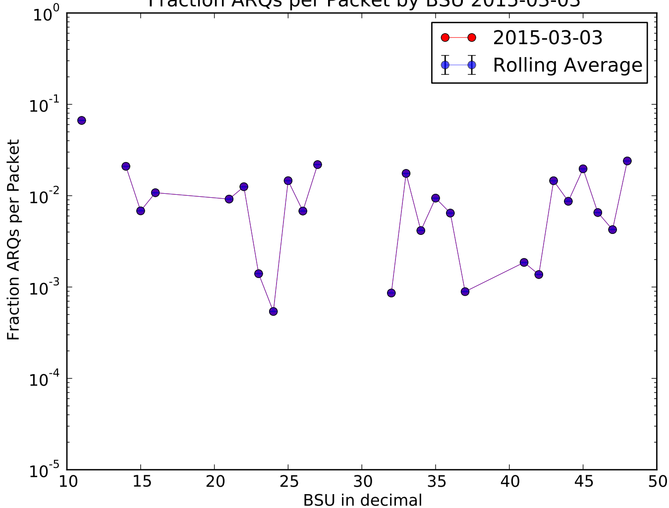
Fraction ARQs per Packet by BSU 2015-03-03
