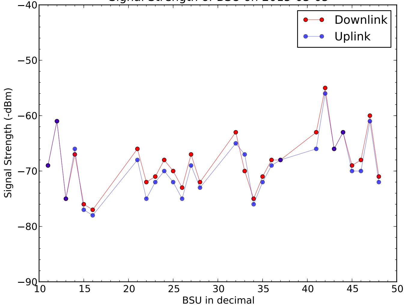
Signal Strength of BSU on 2015-03-05
