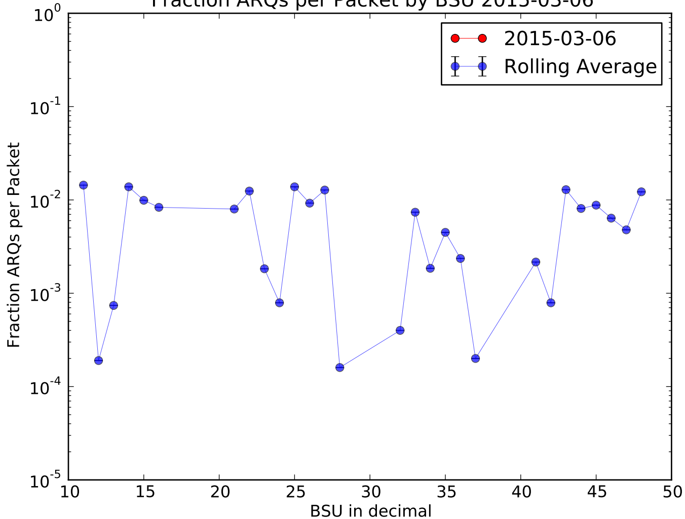
Fraction ARQs per Packet by BSU 2015-03-06
