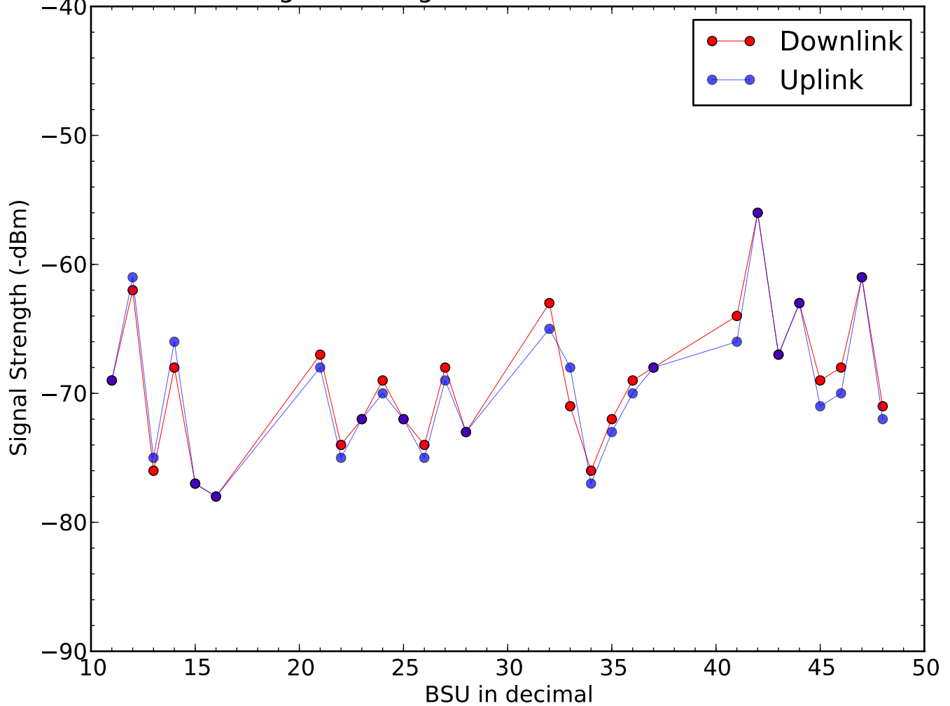
Signal Strength of BSU on 2015-03-12
