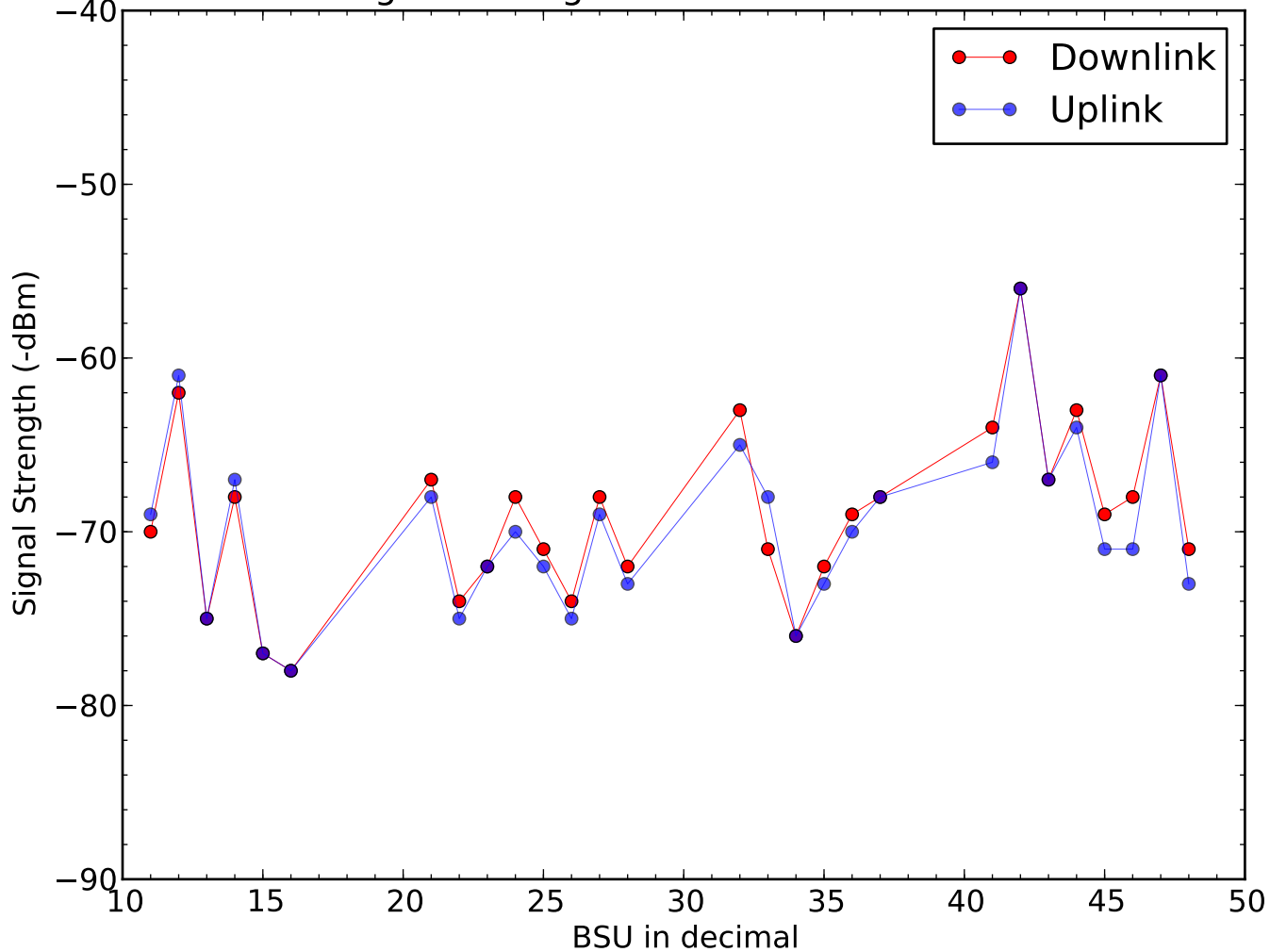
Signal Strength of BSU on 2015-03-13
