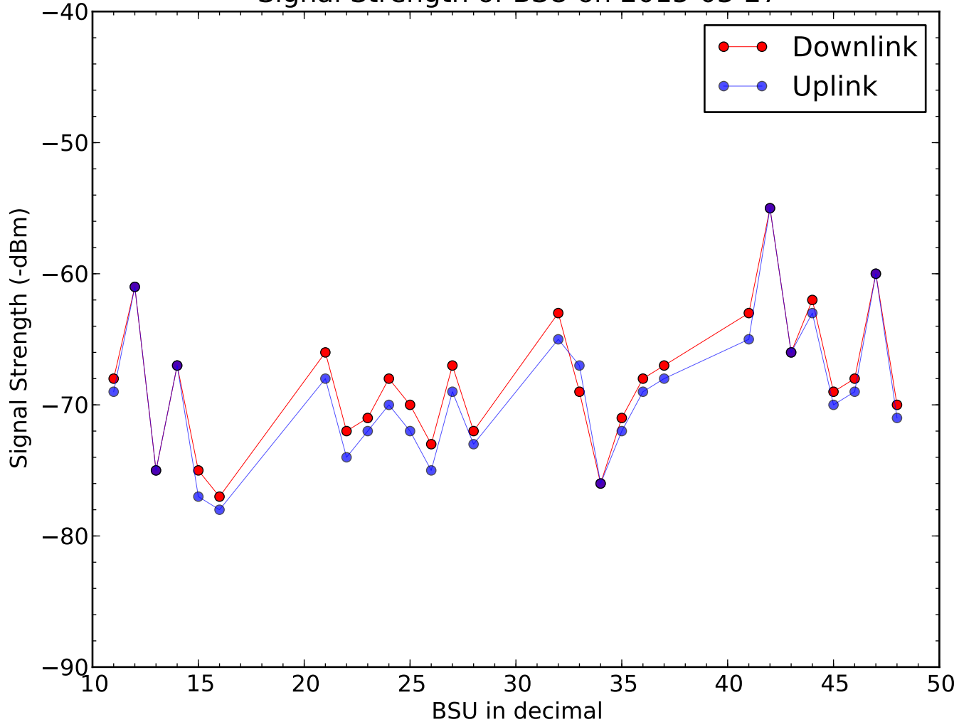
Signal Strength of BSU on 2015-03-27
