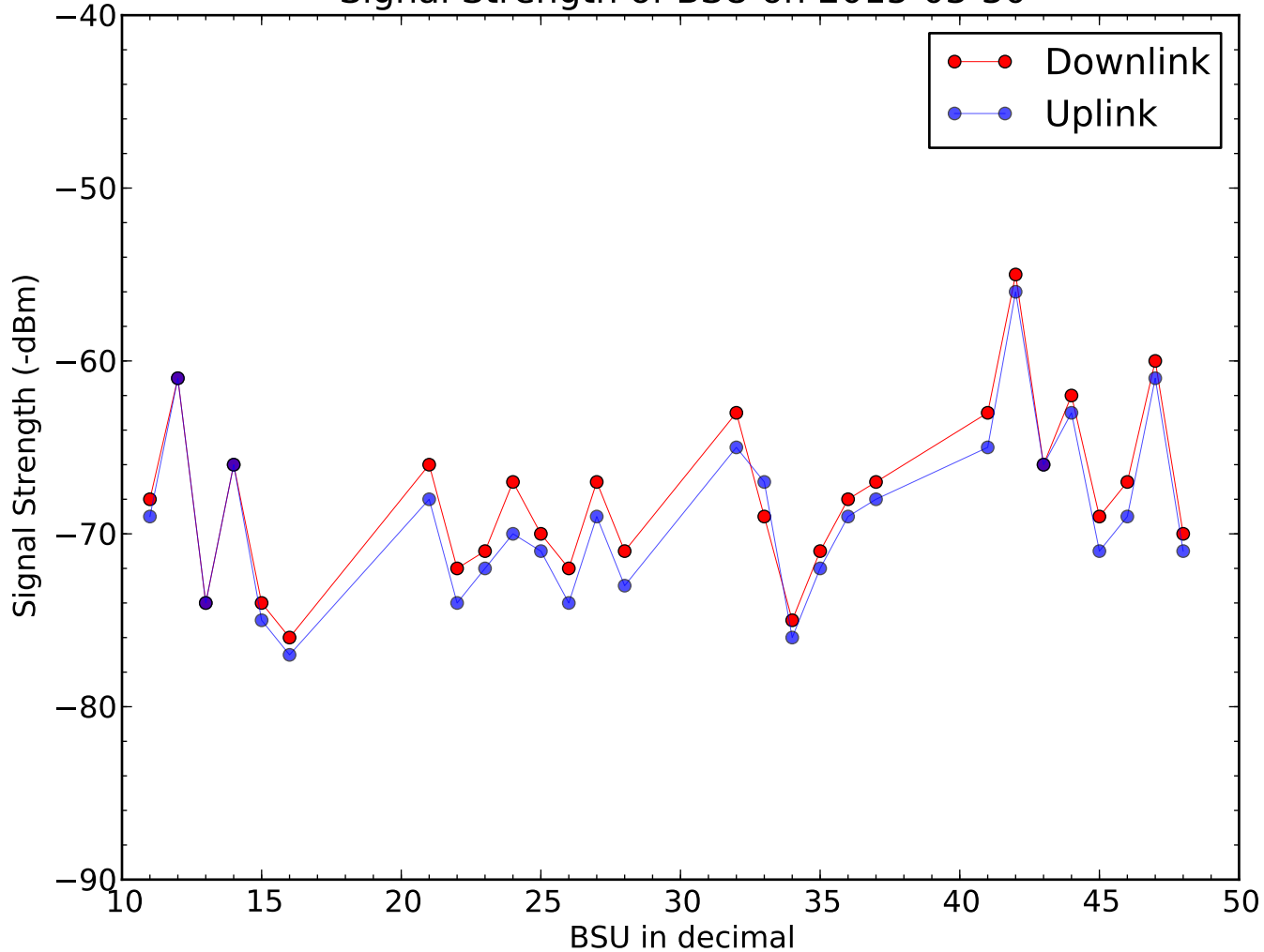
Signal Strength of BSU on 2015-03-30
