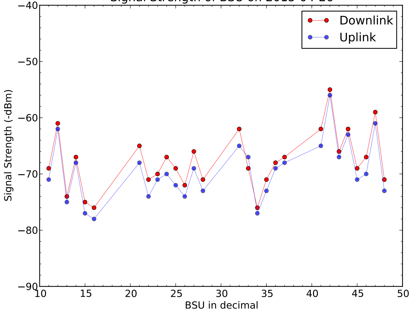
Signal Strength of BSU on 2015-04-26
