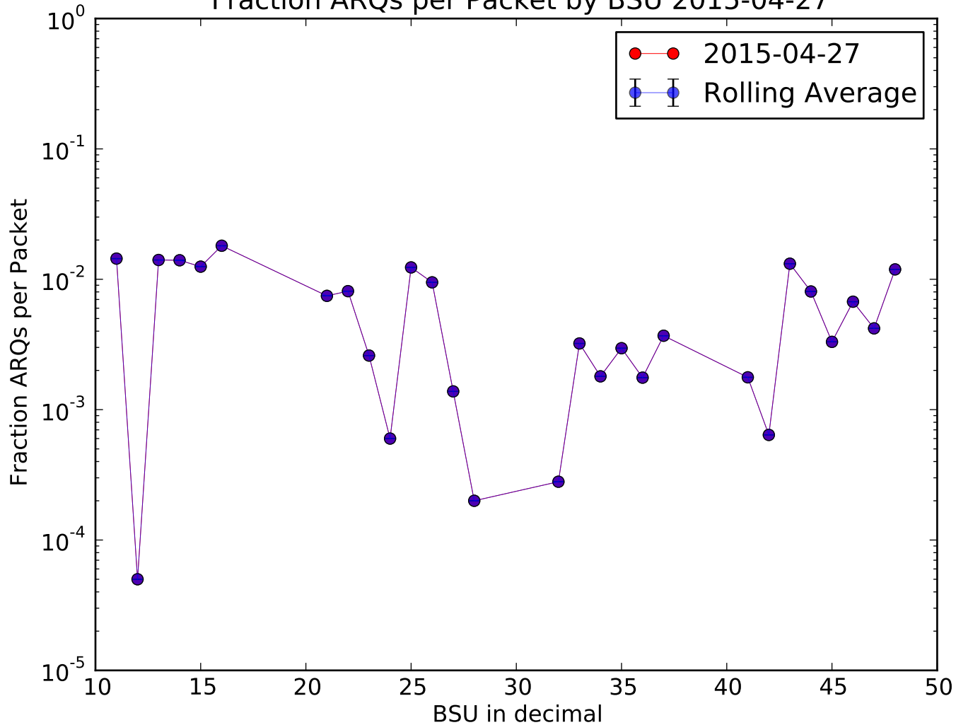
Fraction ARQs per Packet by BSU 2015-04-27
