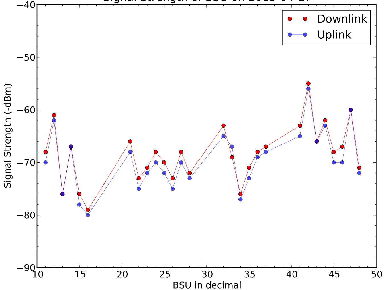
Signal Strength of BSU on 2015-04-27
