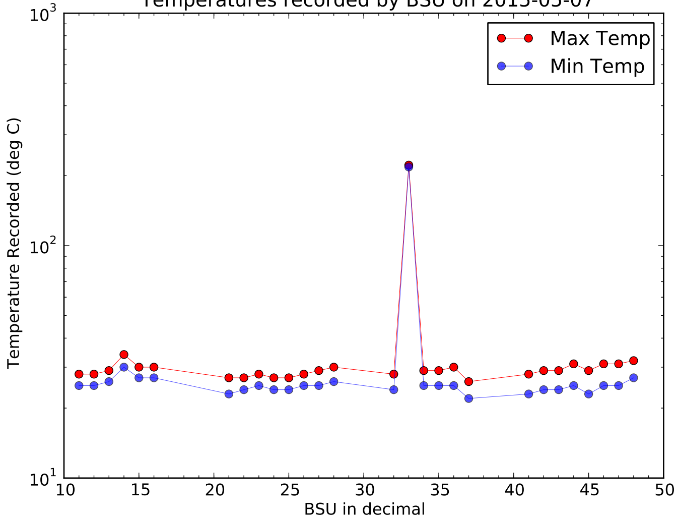
Temperatures recorded by BSU on 2015-05-07
