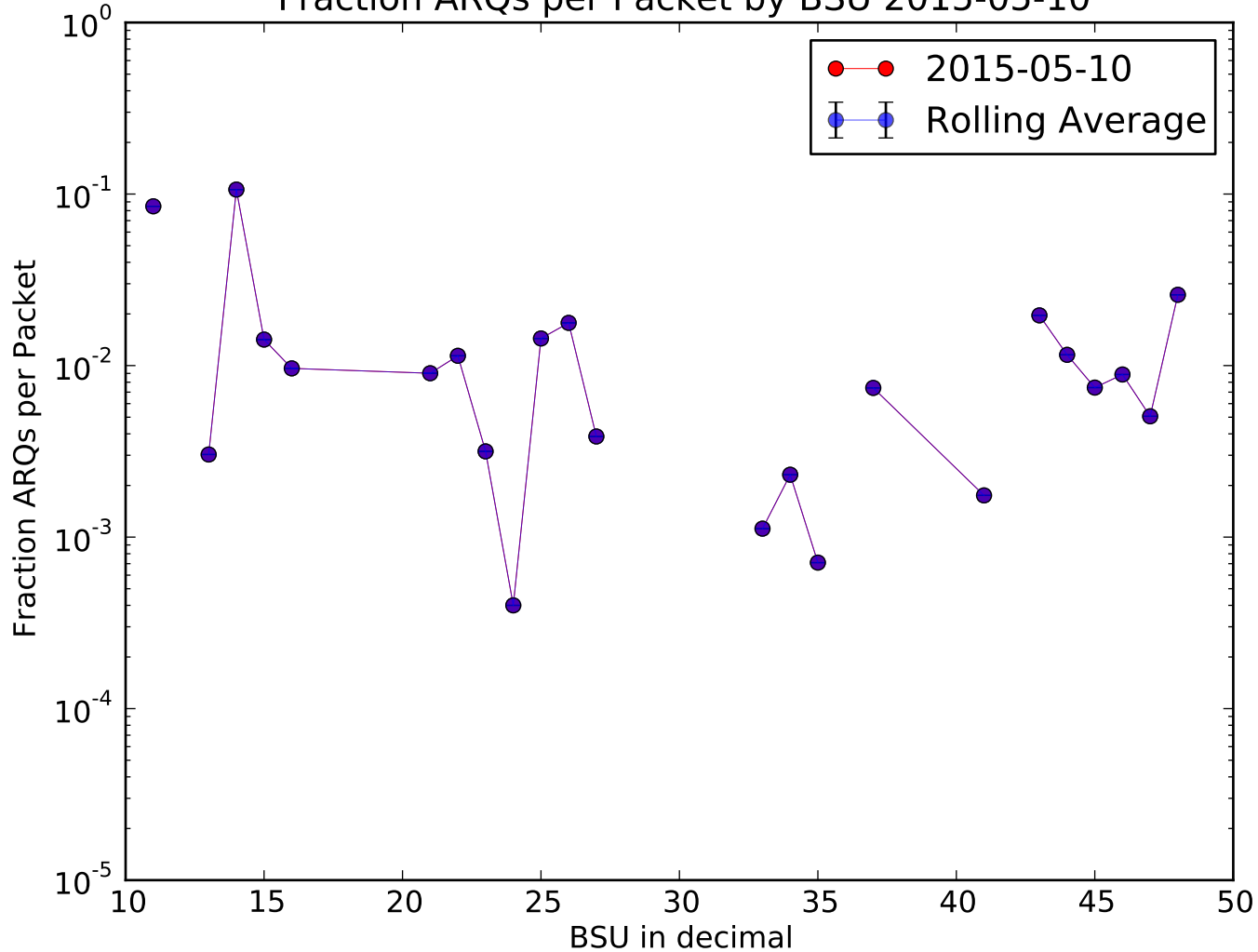
Fraction ARQs per Packet by BSU 2015-05-10
