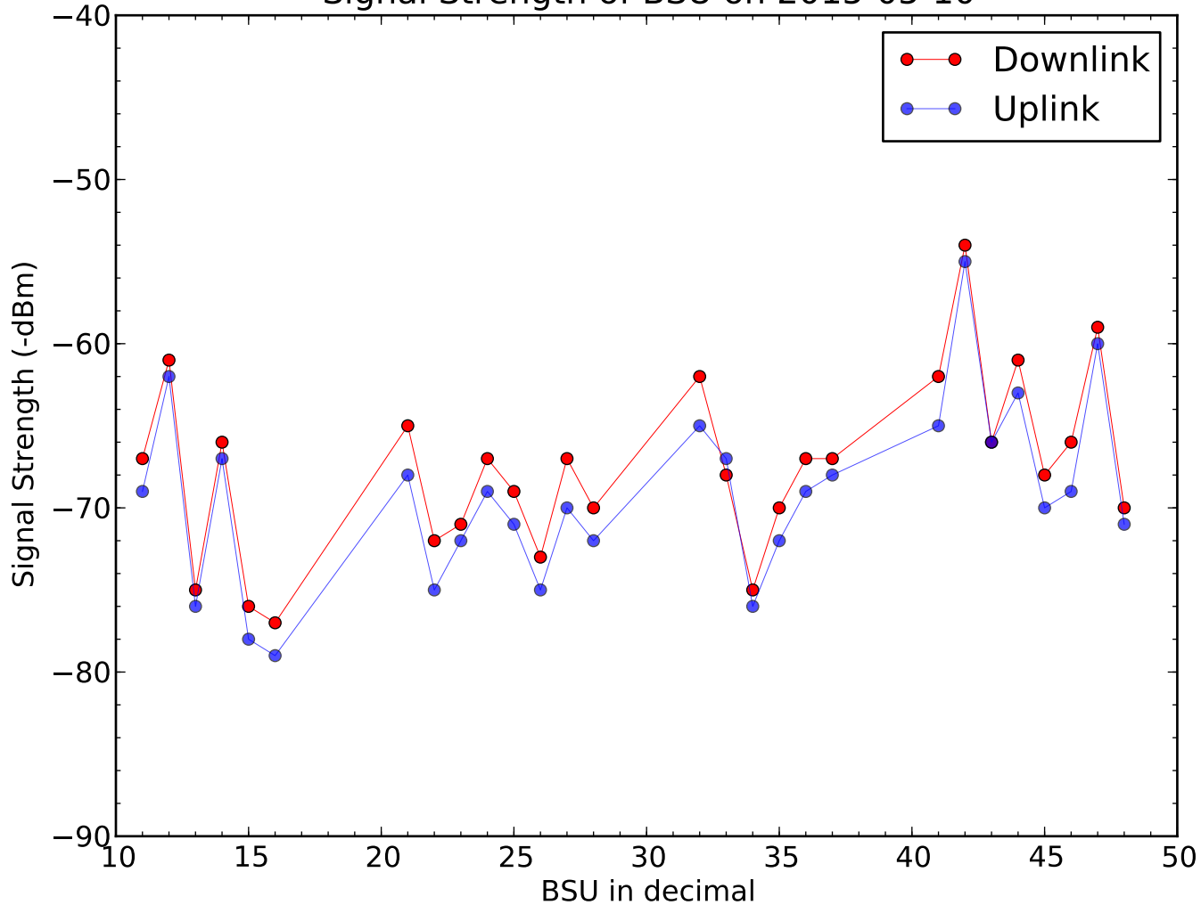
Signal Strength of BSU on 2015-05-10
