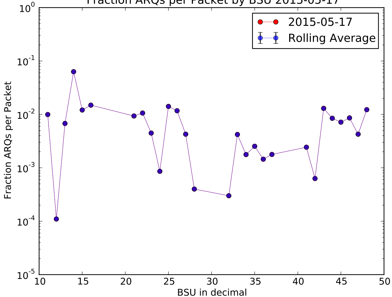
Fraction ARQs per Packet by BSU 2015-05-17
