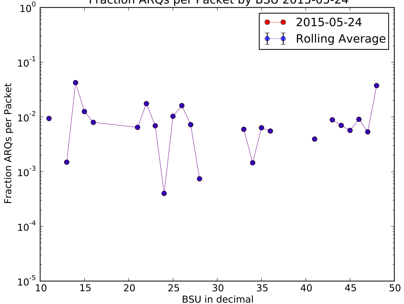
Fraction ARQs per Packet by BSU 2015-05-24
