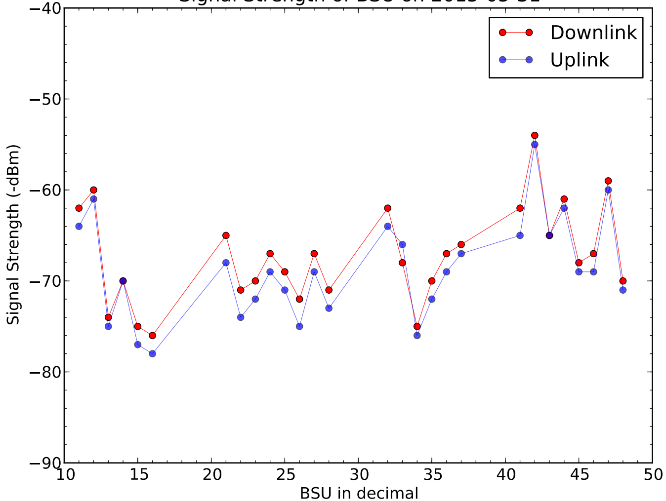
Signal Strength of BSU on 2015-05-31
