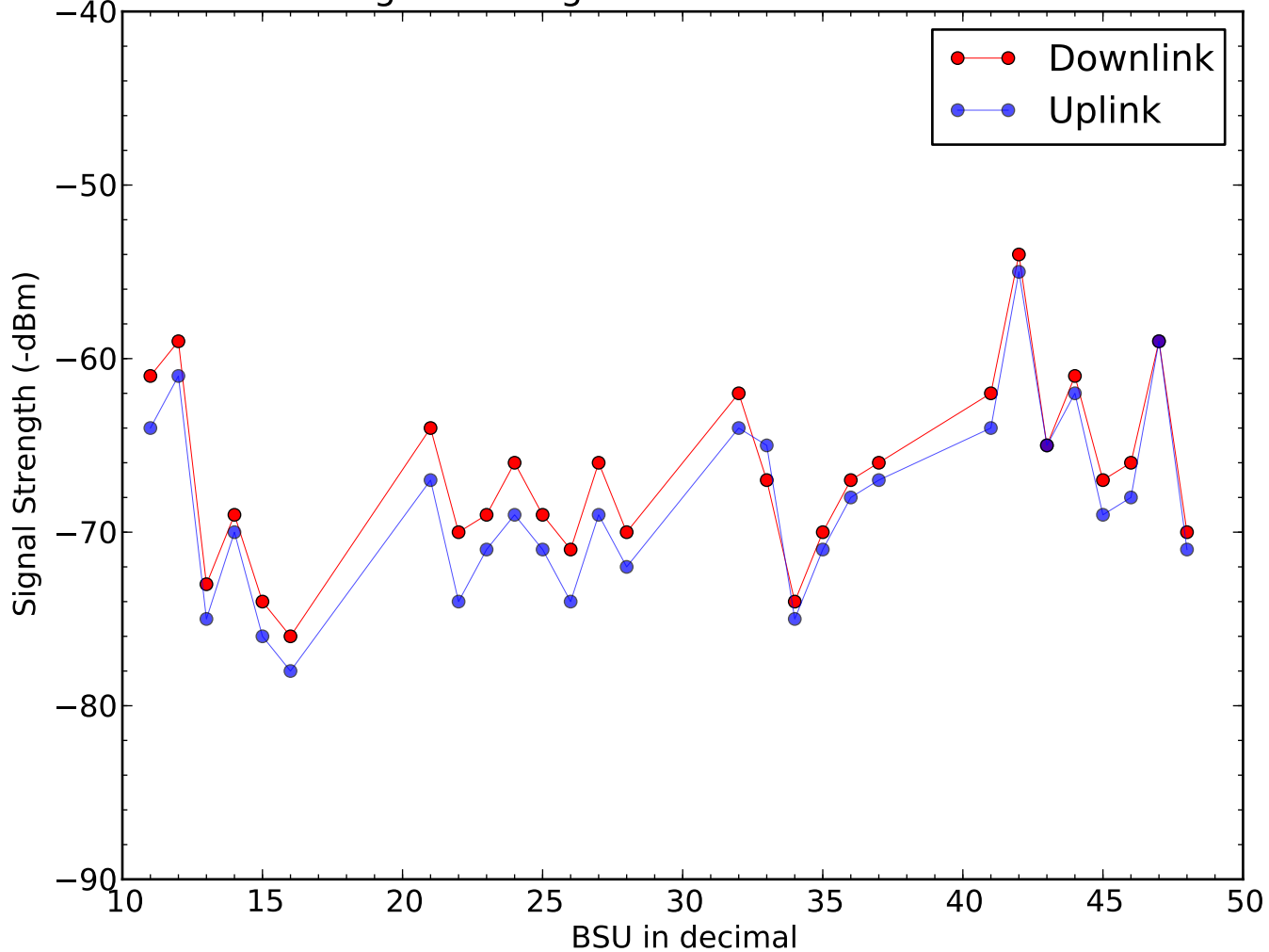
Signal Strength of BSU on 2015-06-19
