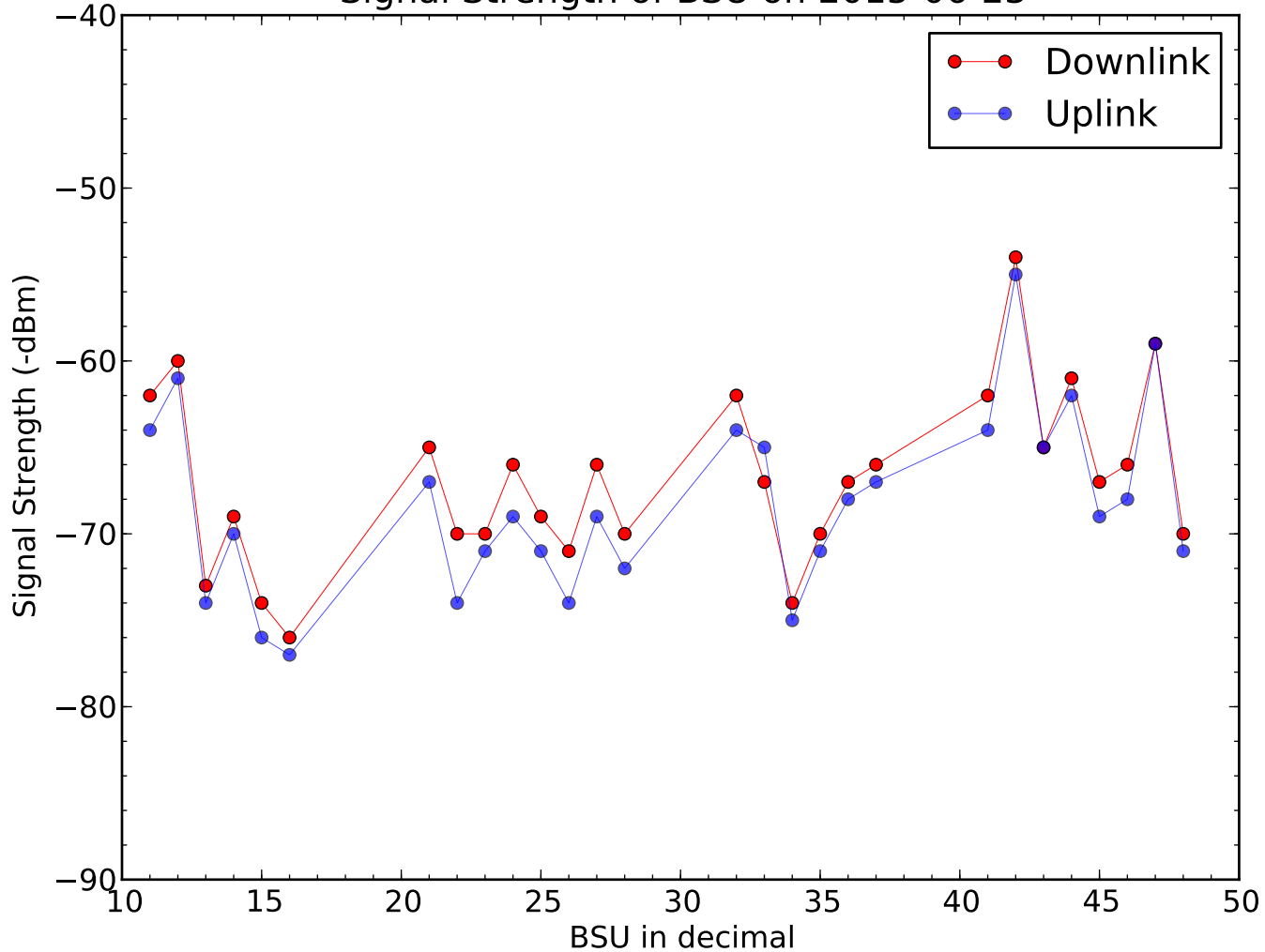
Signal Strength of BSU on 2015-06-23
