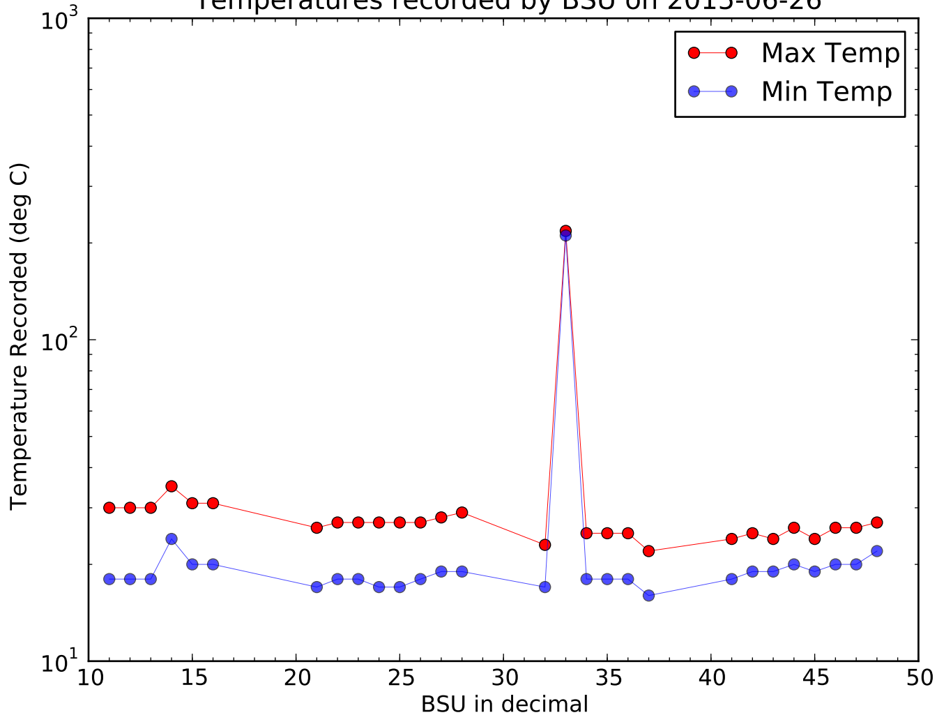
Temperatures recorded by BSU on 2015-06-26
