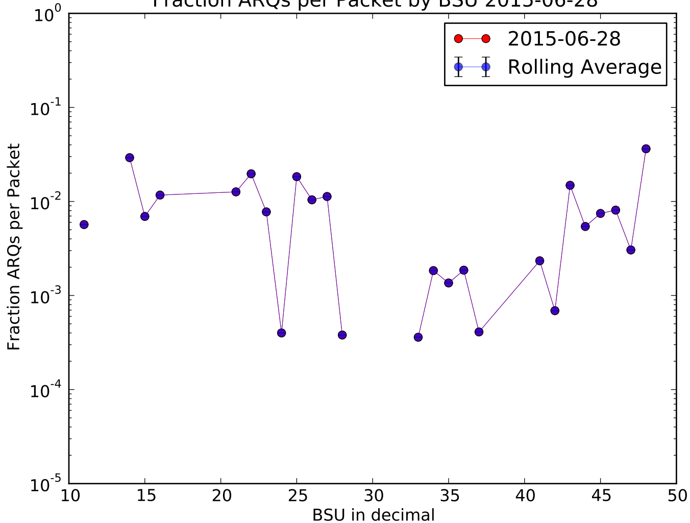
Fraction ARQs per Packet by BSU 2015-06-28
