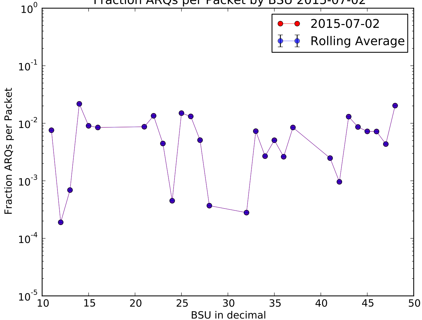
Fraction ARQs per Packet by BSU 2015-07-02
