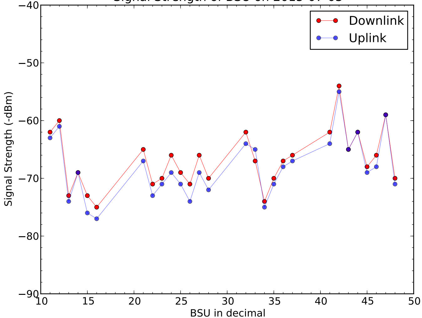
Signal Strength of BSU on 2015-07-03
