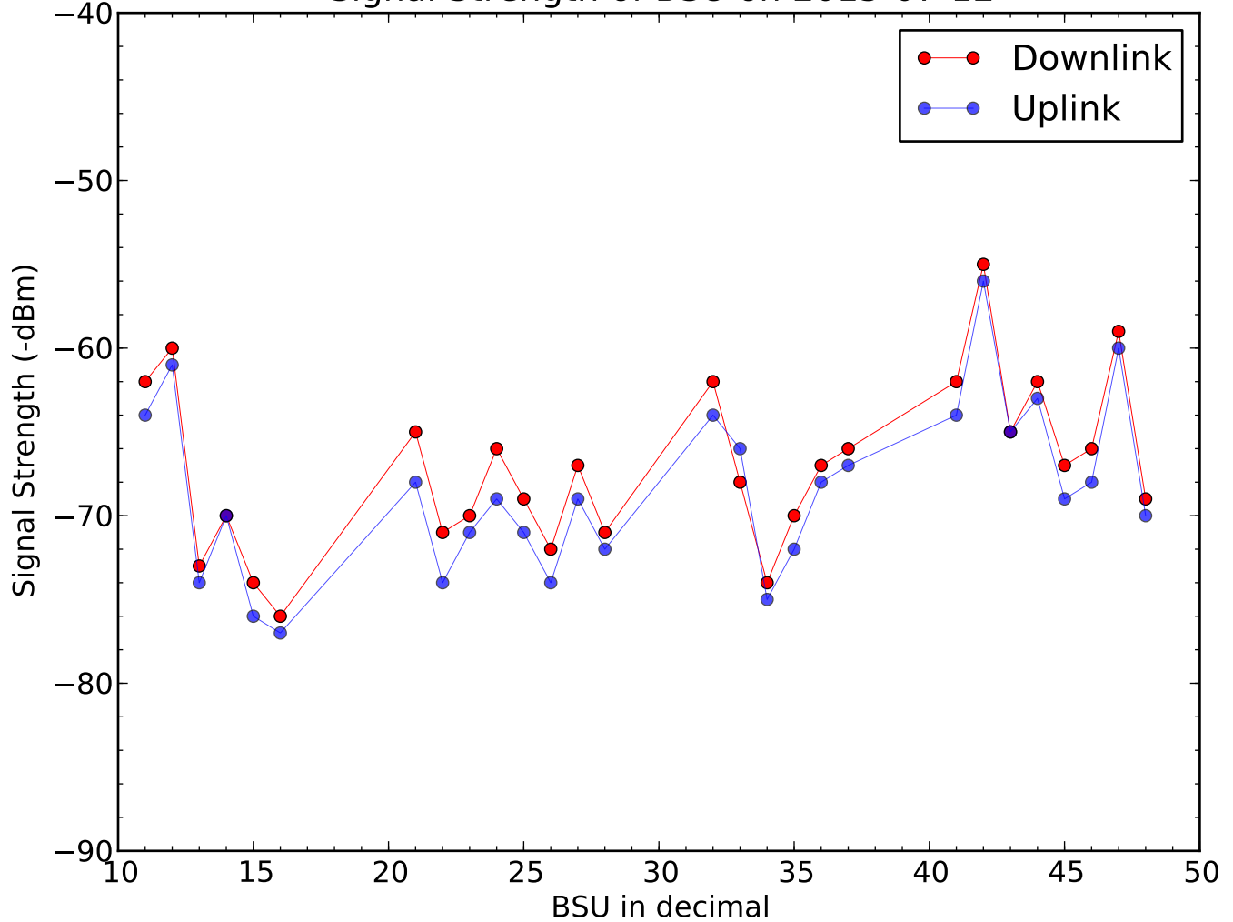
Signal Strength of BSU on 2015-07-12
