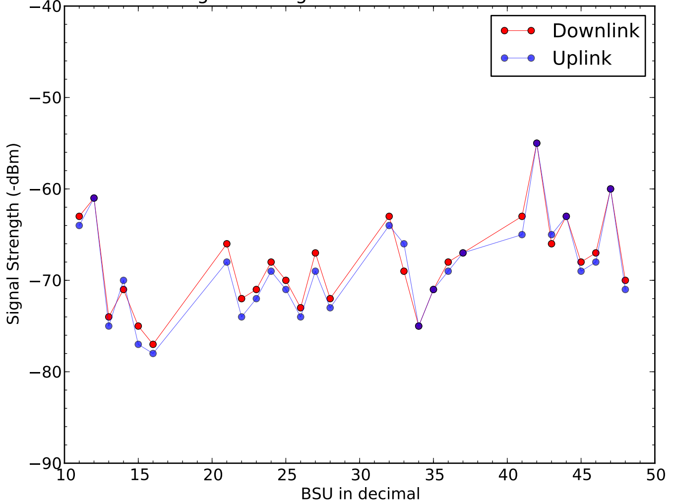
Signal Strength of BSU on 2015-08-05
