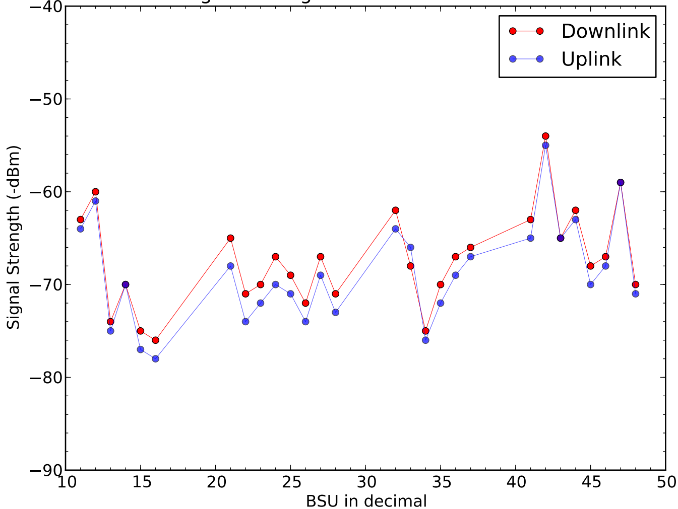
Signal Strength of BSU on 2015-08-26
