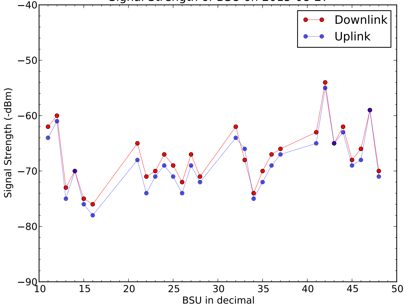
Signal Strength of BSU on 2015-08-27
