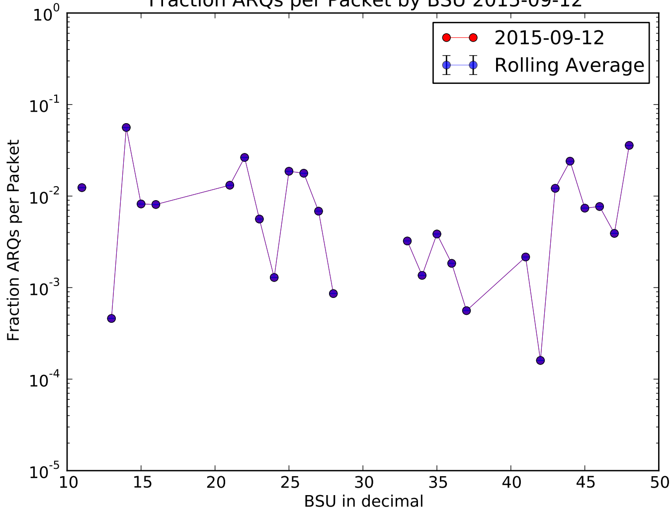
Fraction ARQs per Packet by BSU 2015-09-12
