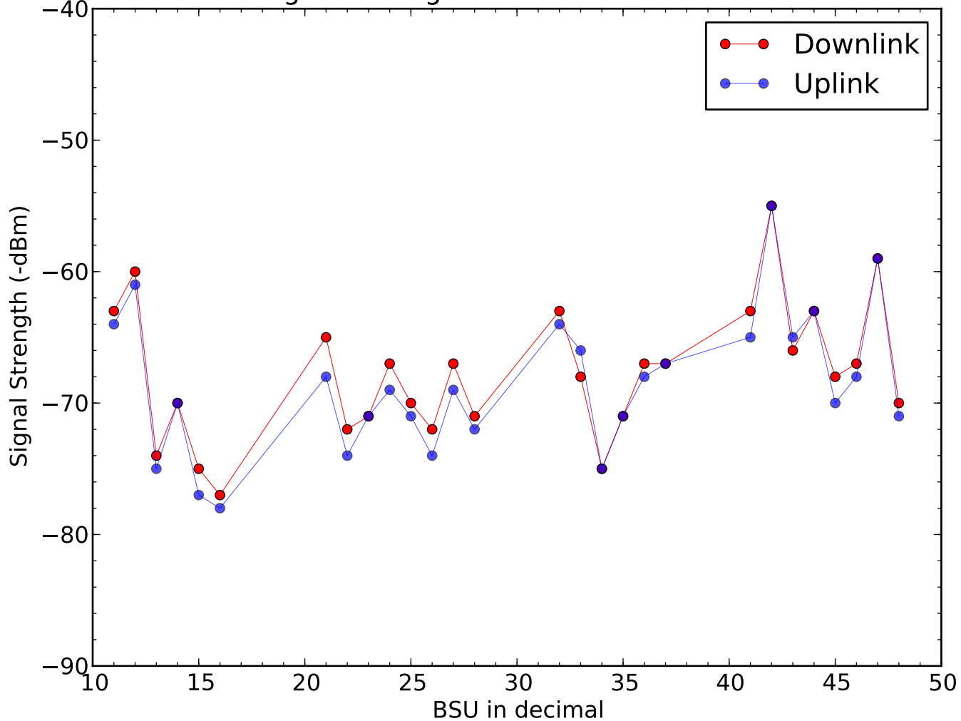
Signal Strength of BSU on 2015-09-25
