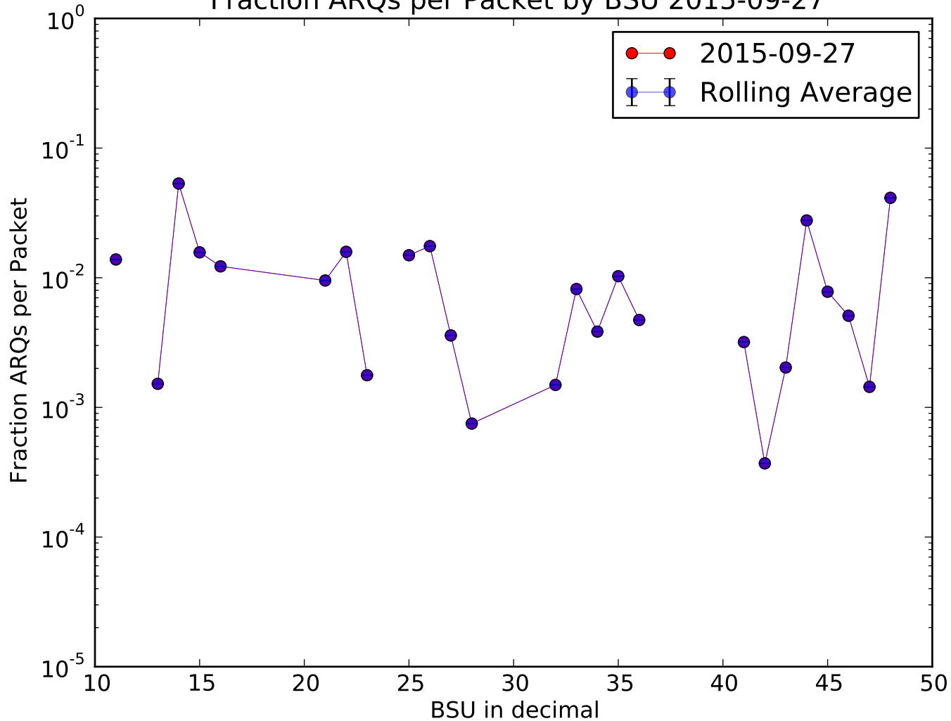
Fraction ARQs per Packet by BSU 2015-09-27
