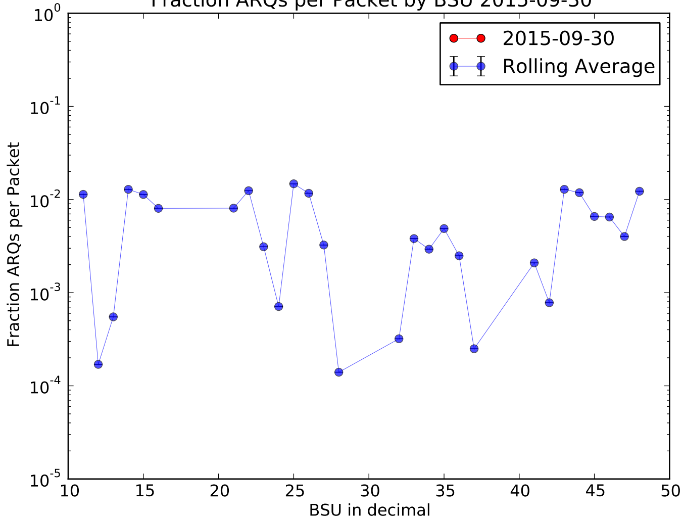
Fraction ARQs per Packet by BSU 2015-09-30
