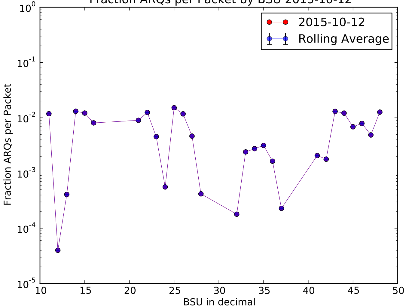
Fraction ARQs per Packet by BSU 2015-10-12
