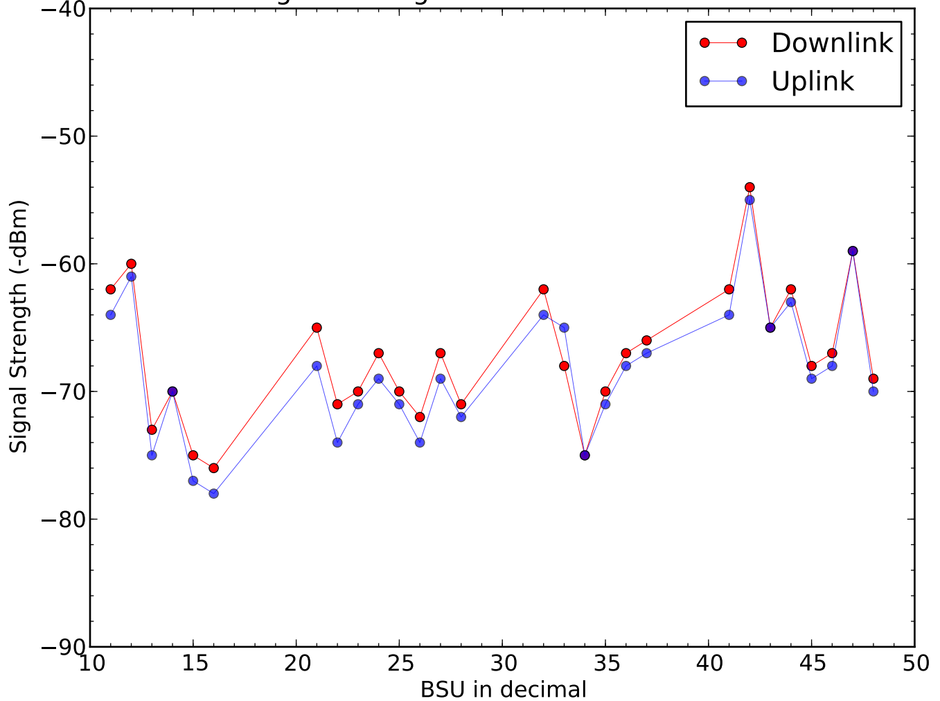
Signal Strength of BSU on 2015-10-12
