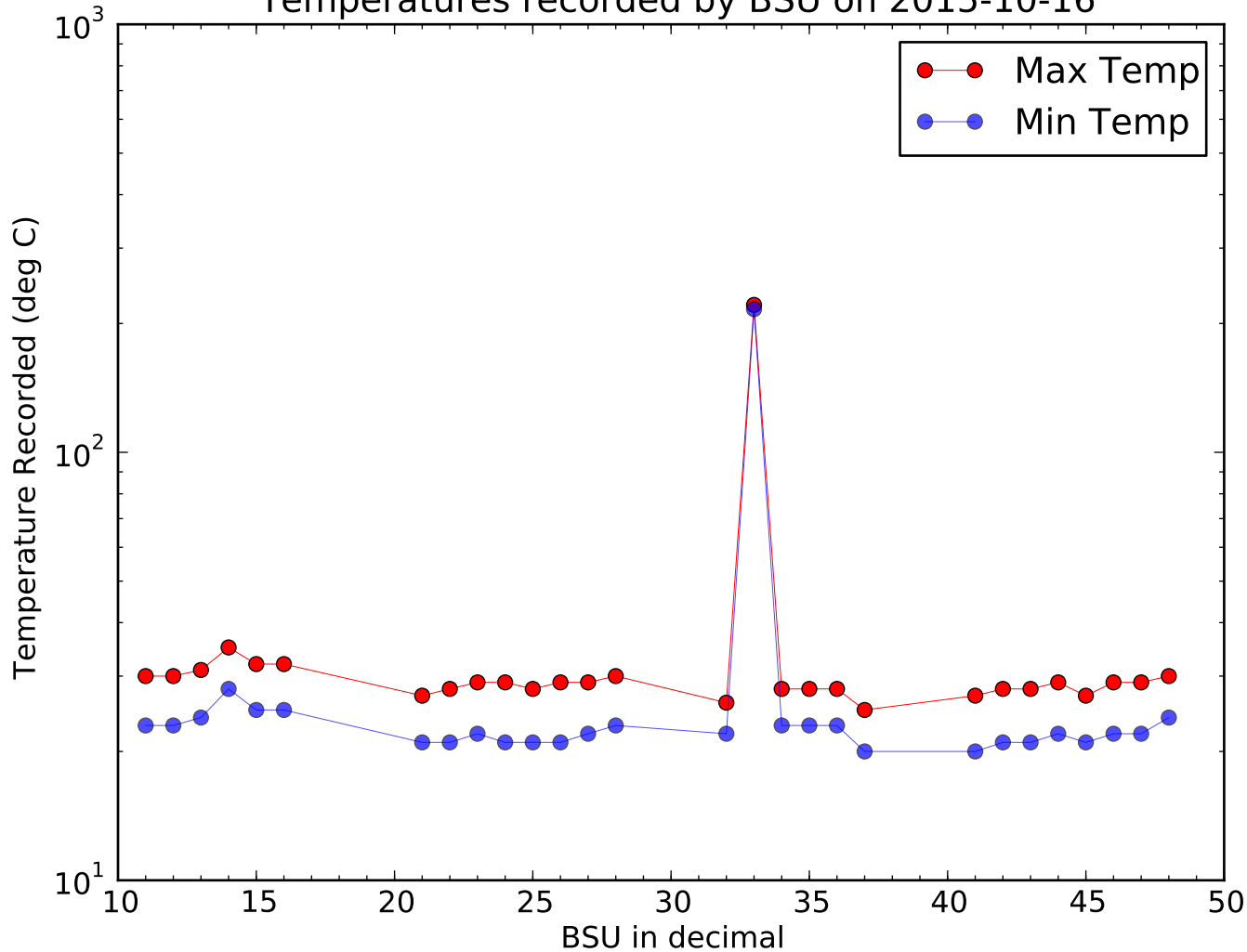
Temperatures recorded by BSU on 2015-10-16
