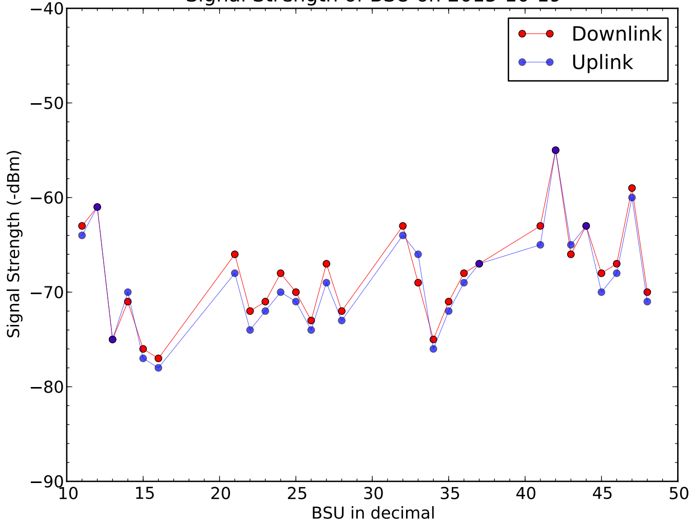
Signal Strength of BSU on 2015-10-19
