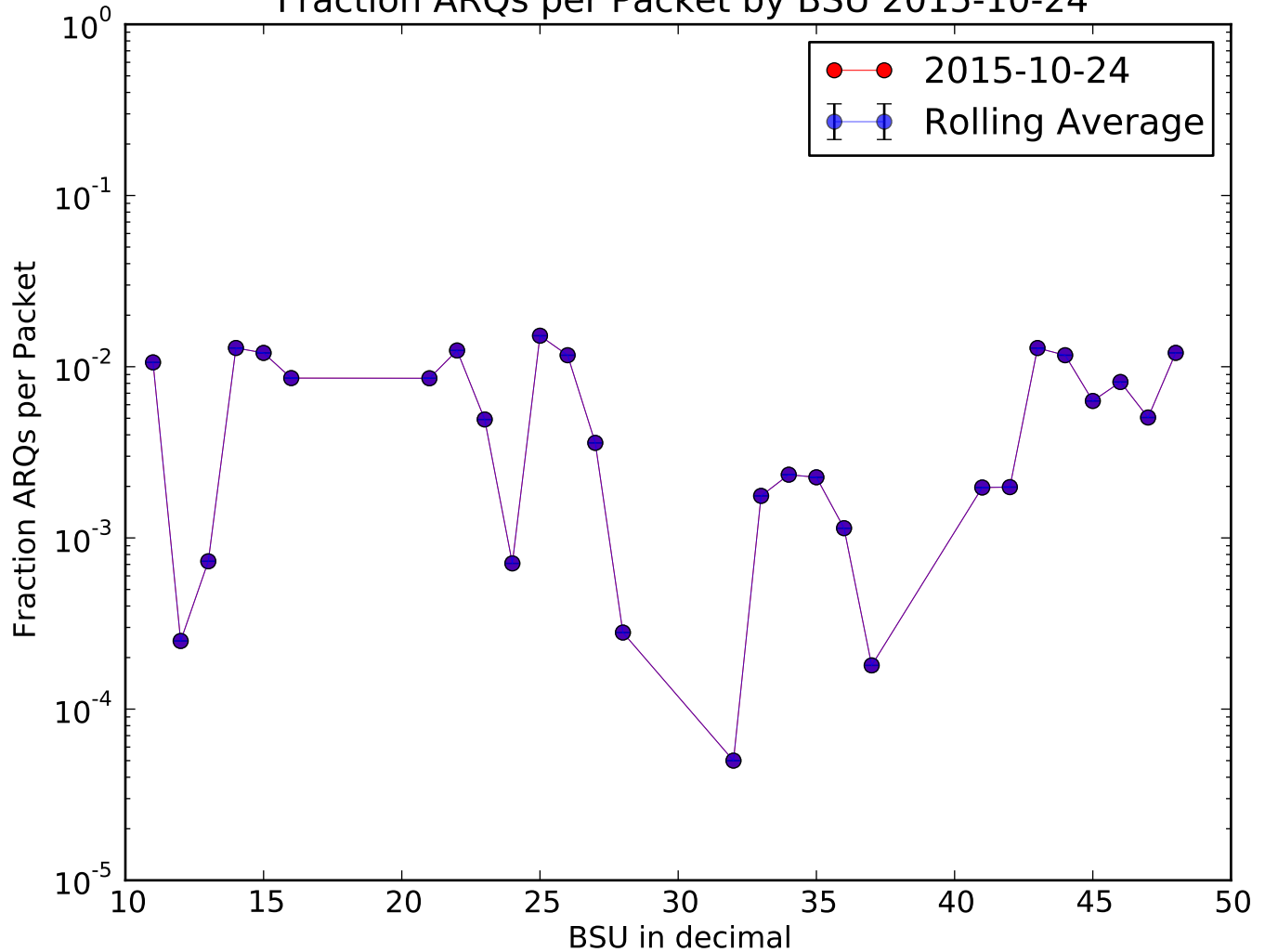
Fraction ARQs per Packet by BSU 2015-10-24
