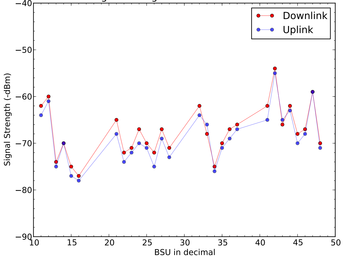
Signal Strength of BSU on 2015-10-24
